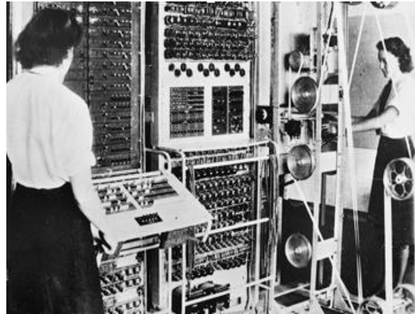
The Colossus electronic digital computer, 1943, FO 850/234
